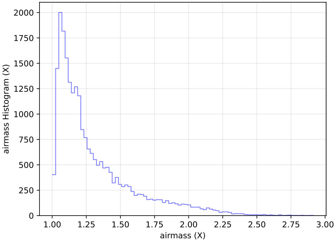
mw_roll_bulge_v3.3_10yrs Yr 1 g band: airmass Histogram
