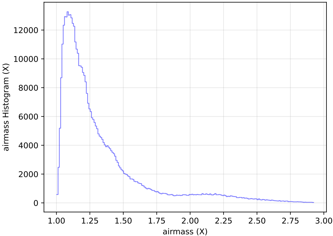
mw_roll_bulge_v3.3_10yrs WFD z band: airmass Histogram
