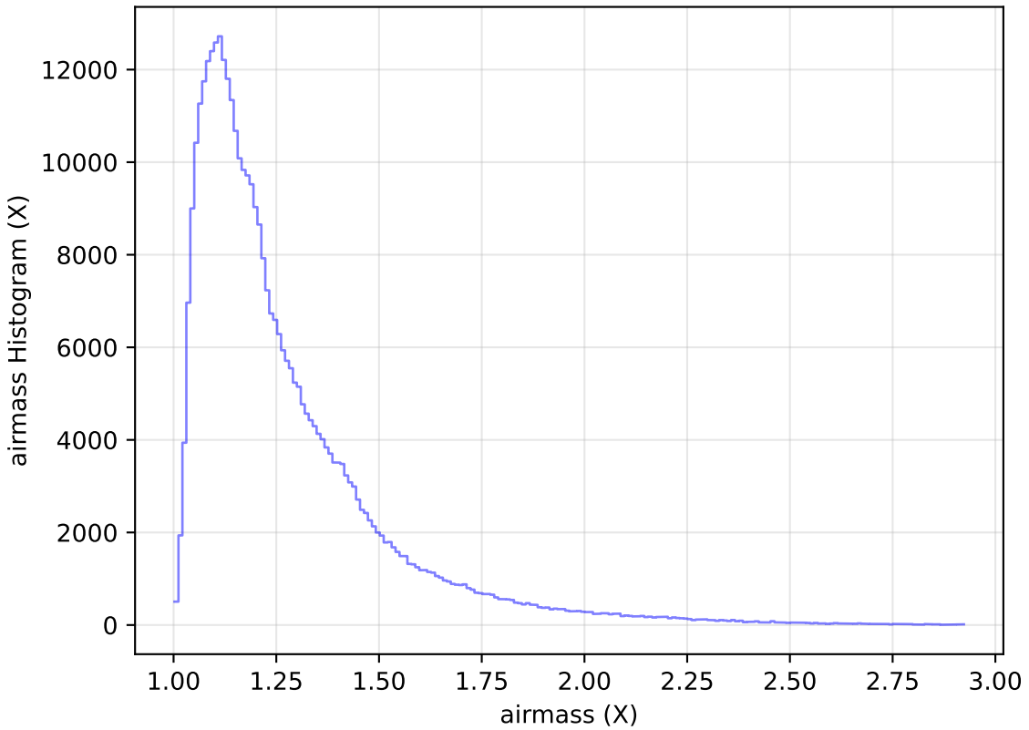
mw_roll_bulge_v3.3_10yrs WFD y band: airmass Histogram
