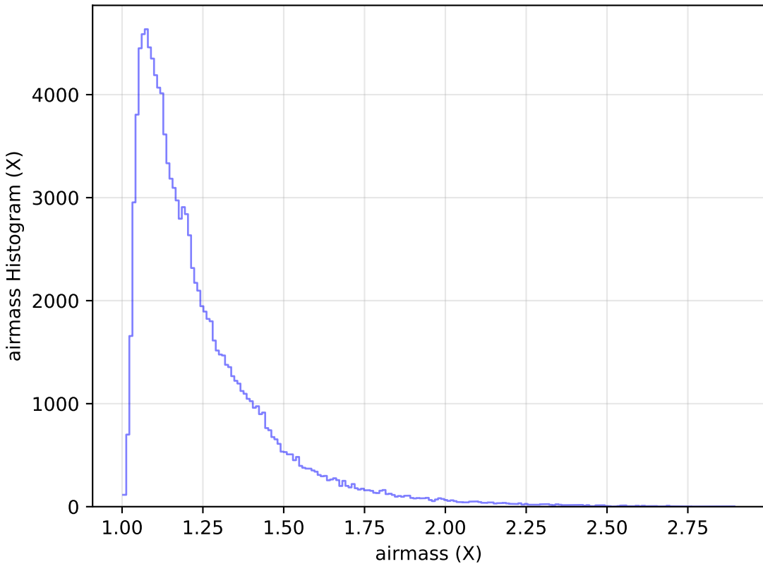
mw_roll_bulge_v3.3_10yrs WFD u band: airmass Histogram
