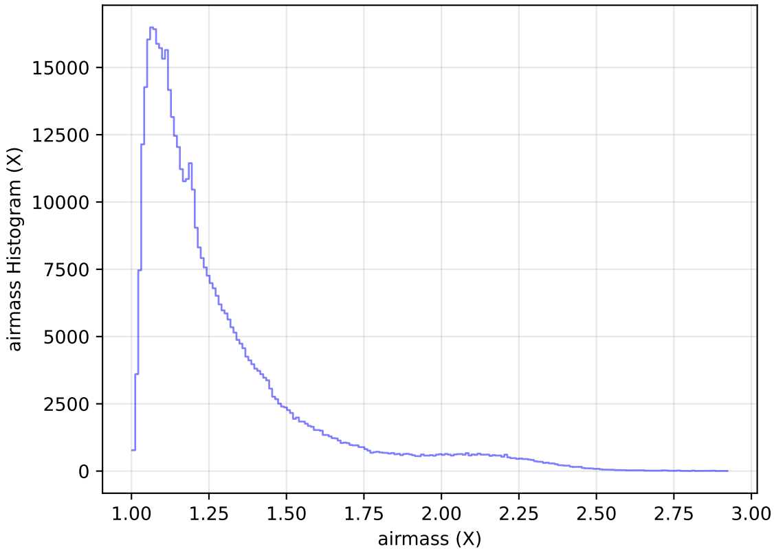
mw_roll_bulge_v3.3_10yrs WFD r band: airmass Histogram
