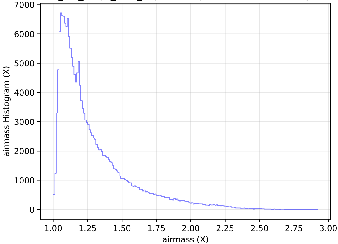
mw_roll_bulge_v3.3_10yrs WFD g band: airmass Histogram
