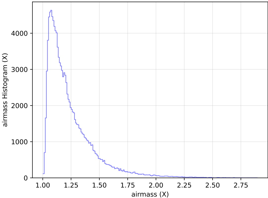
mw_roll_bulge_v3.3_10yrs All sky u band: airmass Histogram
