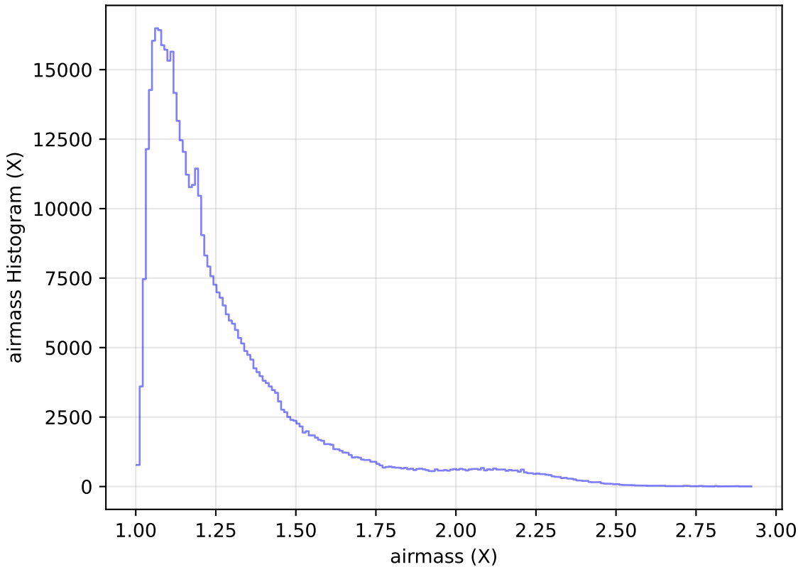
mw_roll_bulge_v3.3_10yrs All sky r band: airmass Histogram
