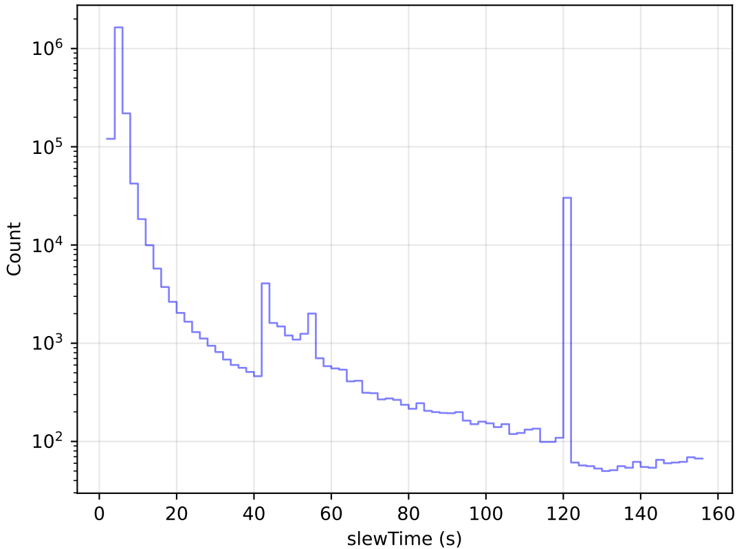
mw_roll_bulge_v3.3_10yrs All visits: Slew Time Histogram
