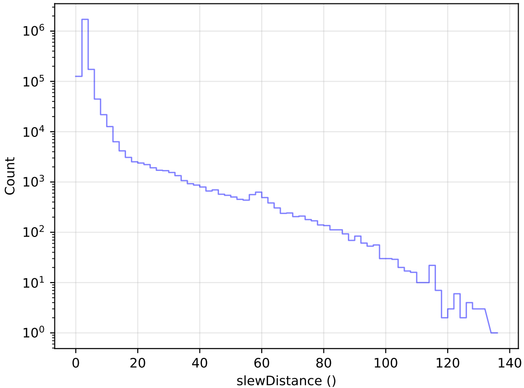
mw_roll_bulge_v3.3_10yrs All visits: Slew Distance Histogram
