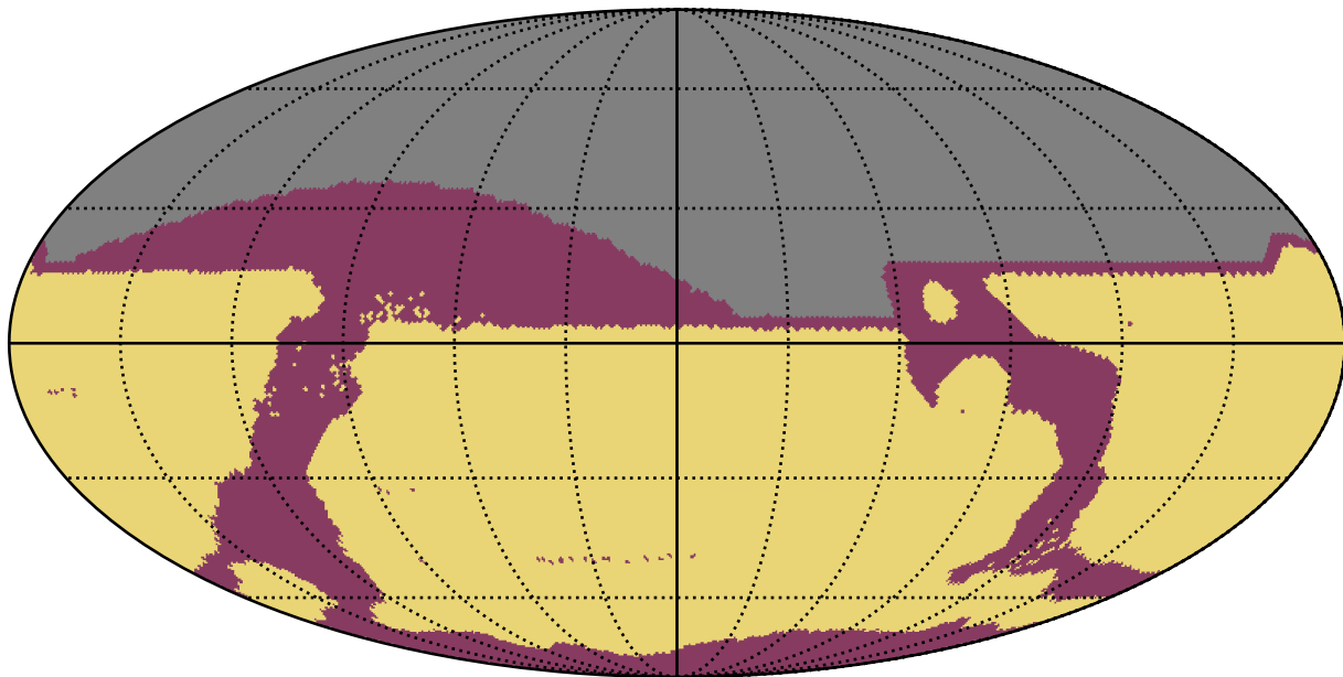
mw_roll_bulge_v3.3_10yrs All sky: RapidRevisits
