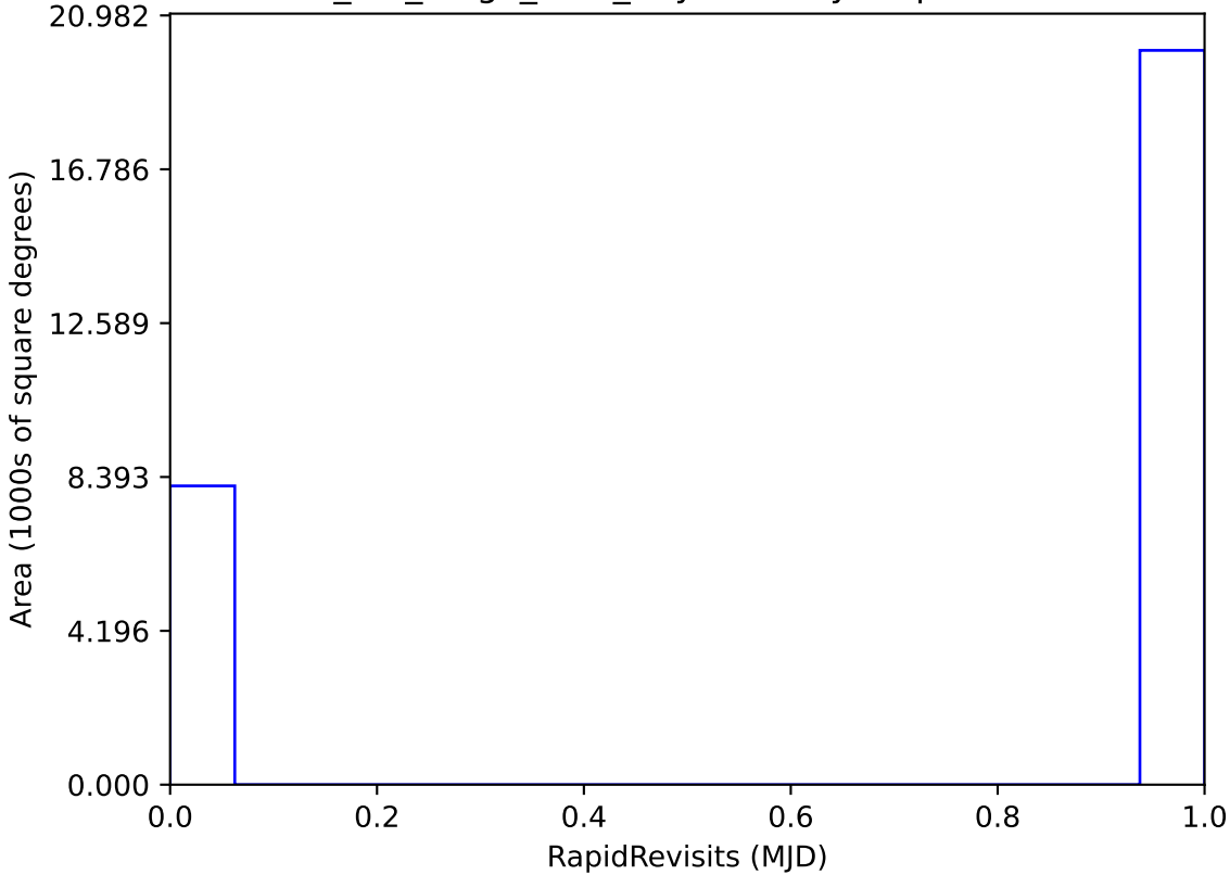
mw_roll_bulge_v3.3_10yrs All sky: RapidRevisits
