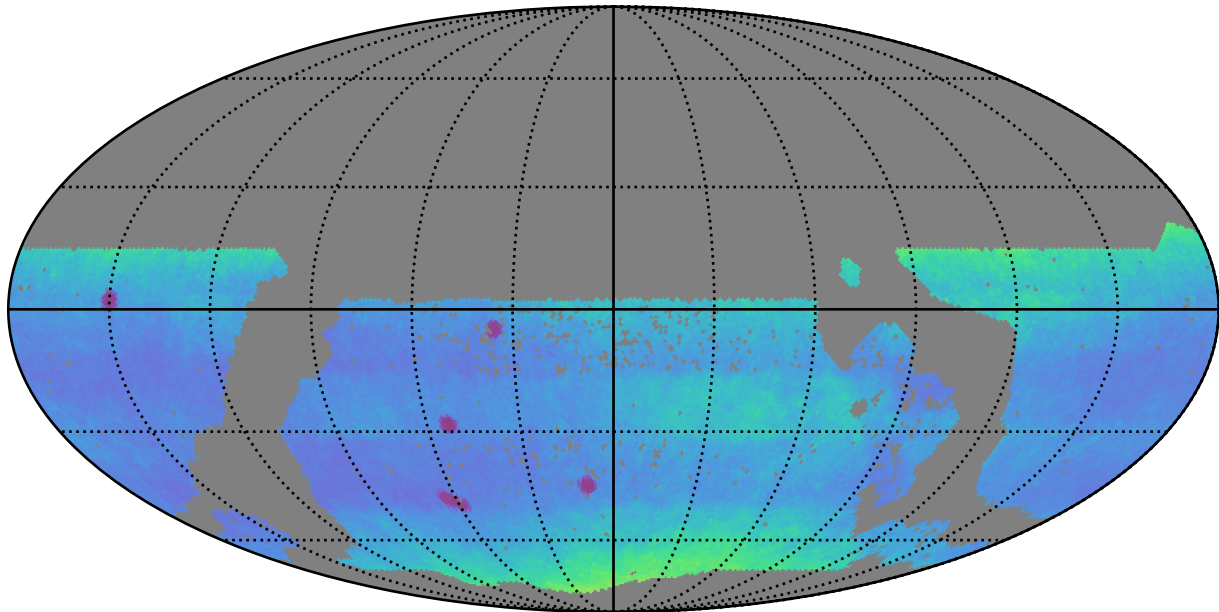
mw_roll_bulge_v3.3_10yrs WFD: Proper Motion Uncert @ 24.0
