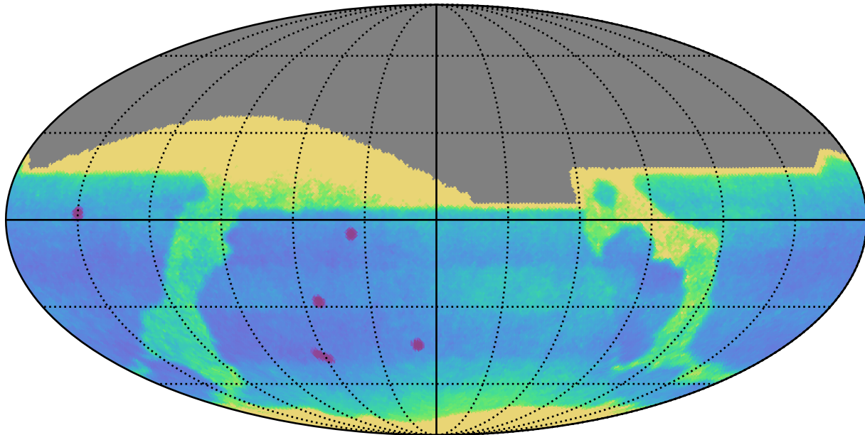
mw_roll_bulge_v3.3_10yrs All sky: Proper Motion Uncert @ 24.0
