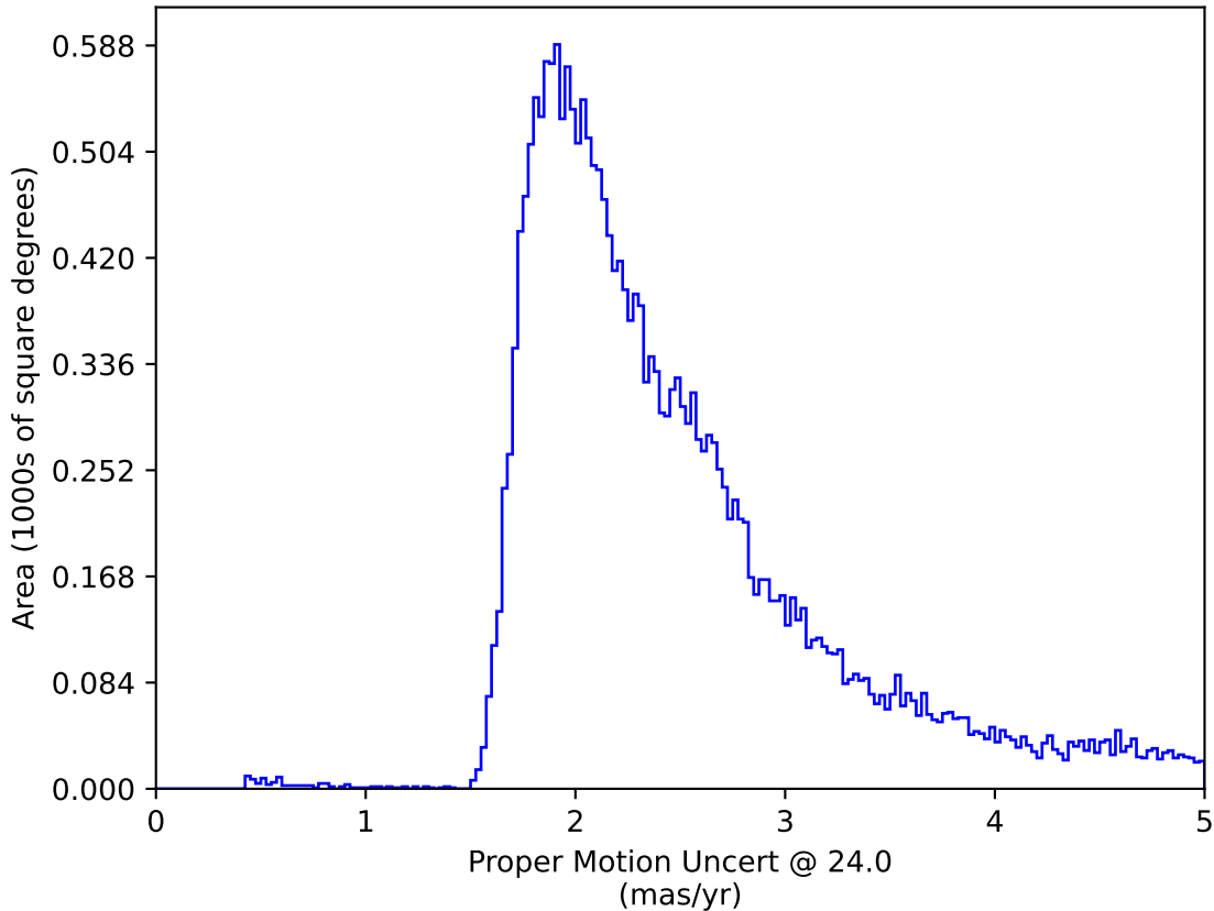
mw_roll_bulge_v3.3_10yrs All sky: Proper Motion Uncert @ 24.0
