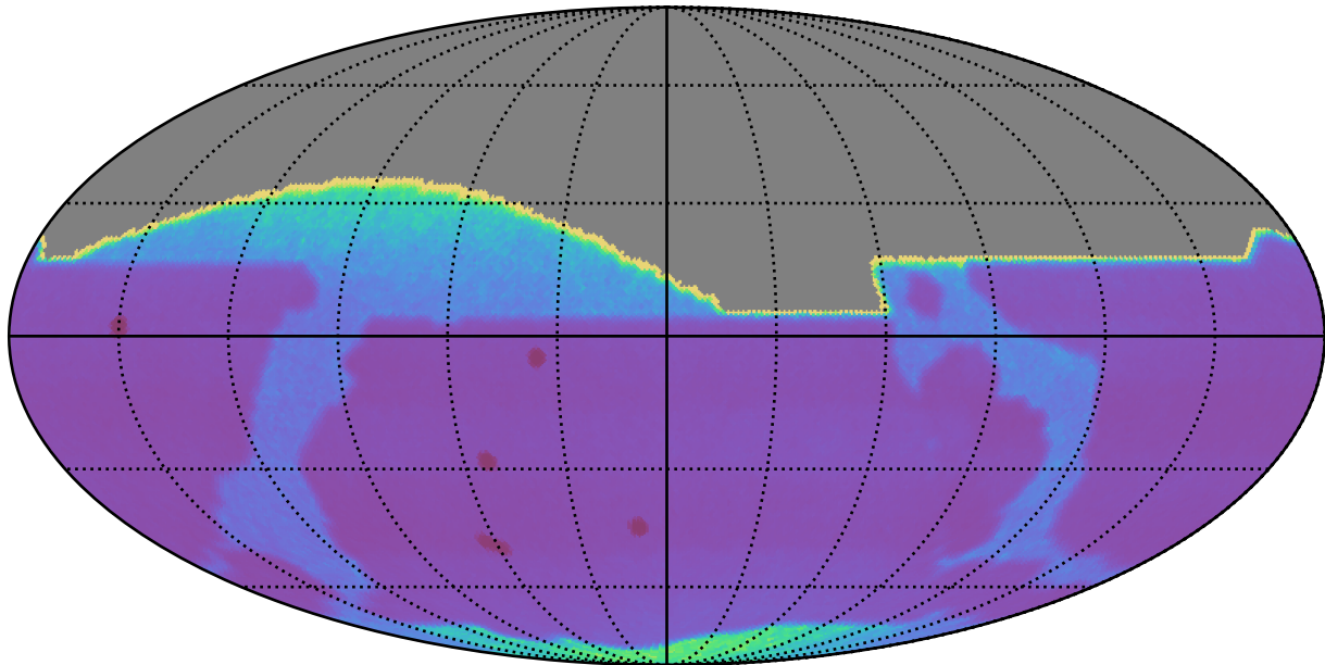
mw_roll_bulge_v3.3_10yrs All sky: Proper Motion Uncert @ 20.5
