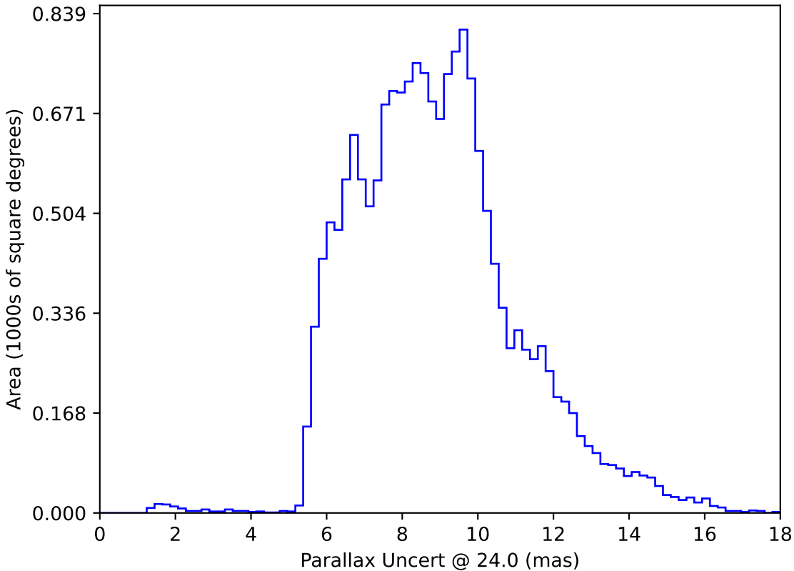
mw_roll_bulge_v3.3_10yrs WFD: Parallax Uncert @ 24.0
