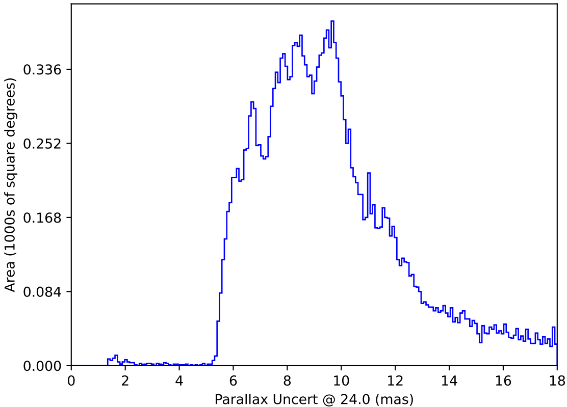
mw_roll_bulge_v3.3_10yrs All sky: Parallax Uncert @ 24.0
