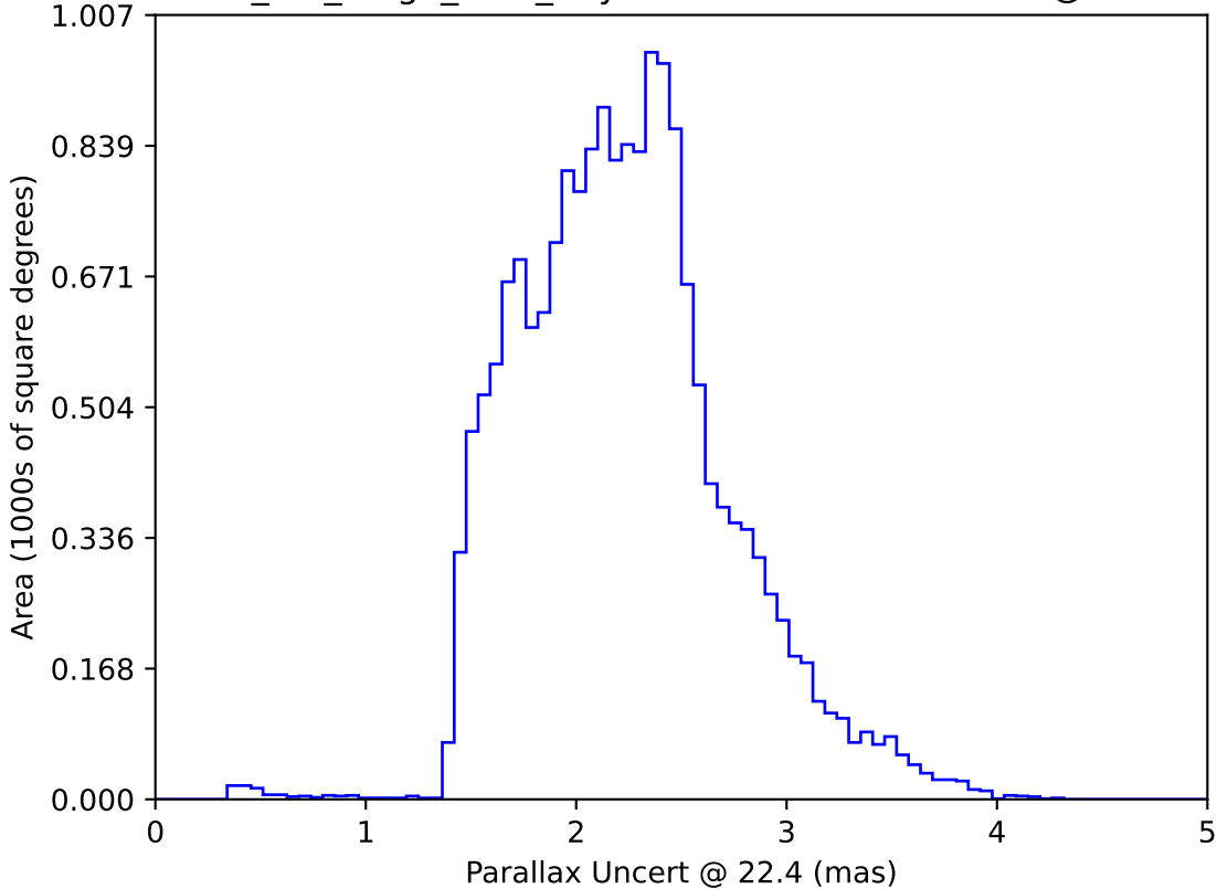
mw_roll_bulge_v3.3_10yrs WFD: Parallax Uncert @ 22.4
