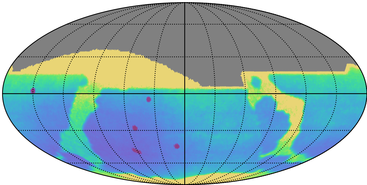
mw_roll_bulge_v3.3_10yrs All sky: Parallax Uncert @ 22.4
