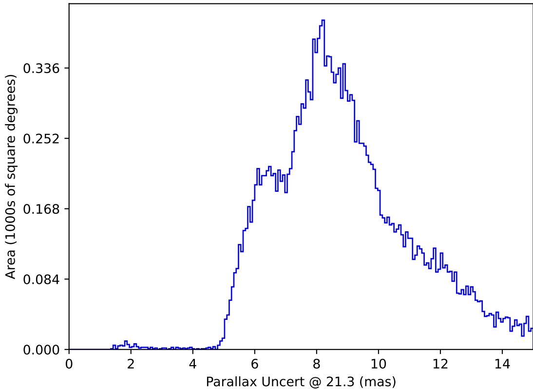
mw_roll_bulge_v3.3_10yrs All sky y band only: Parallax Uncert @ 21.3
