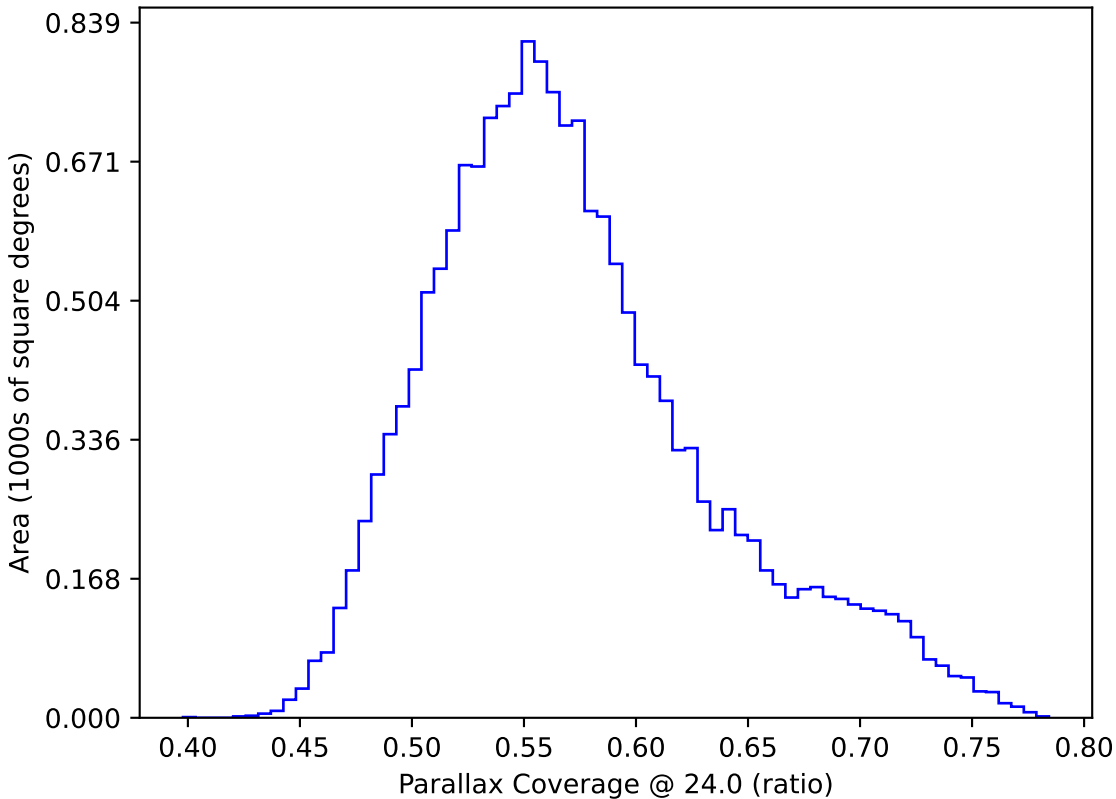
mw_roll_bulge_v3.3_10yrs WFD: Parallax Coverage @ 24.0
