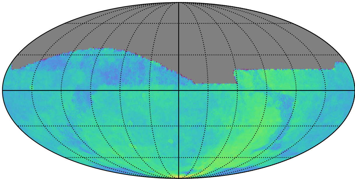
mw_roll_bulge_v3.3_10yrs All sky: Parallax Coverage @ 24.0
