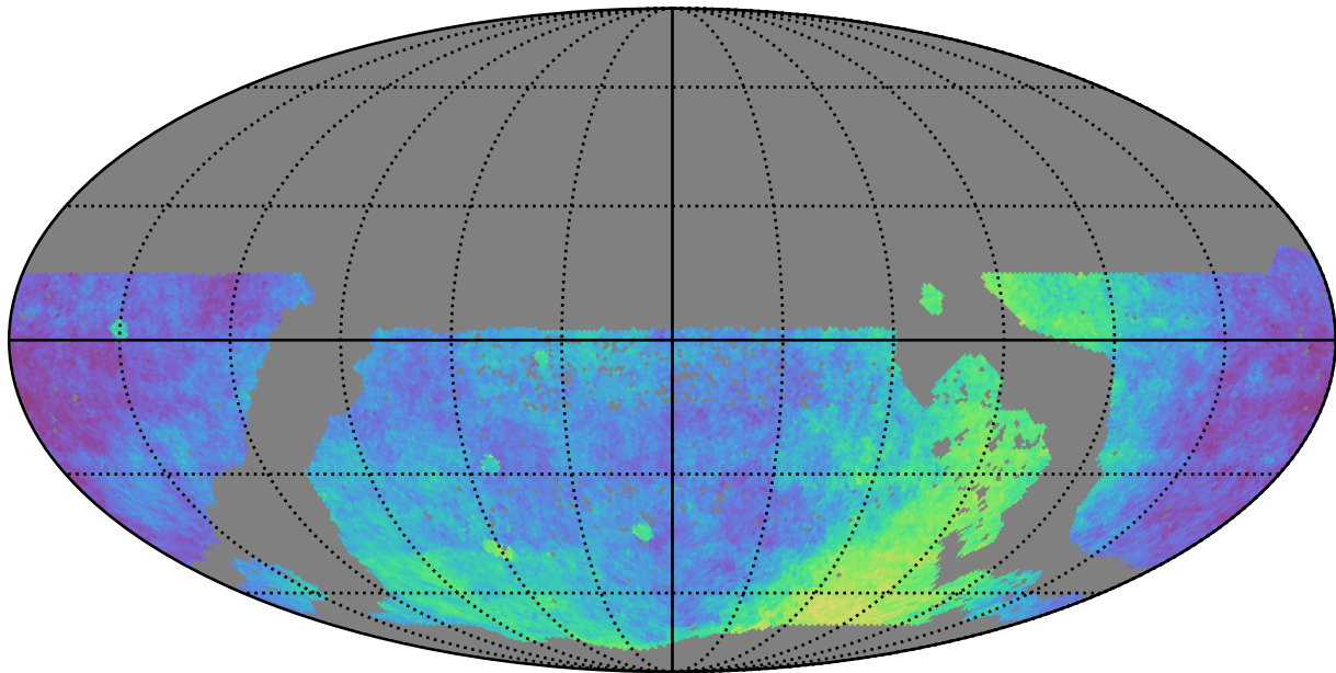
mw_roll_bulge_v3.3_10yrs WFD: Parallax Coverage @ 22.4
