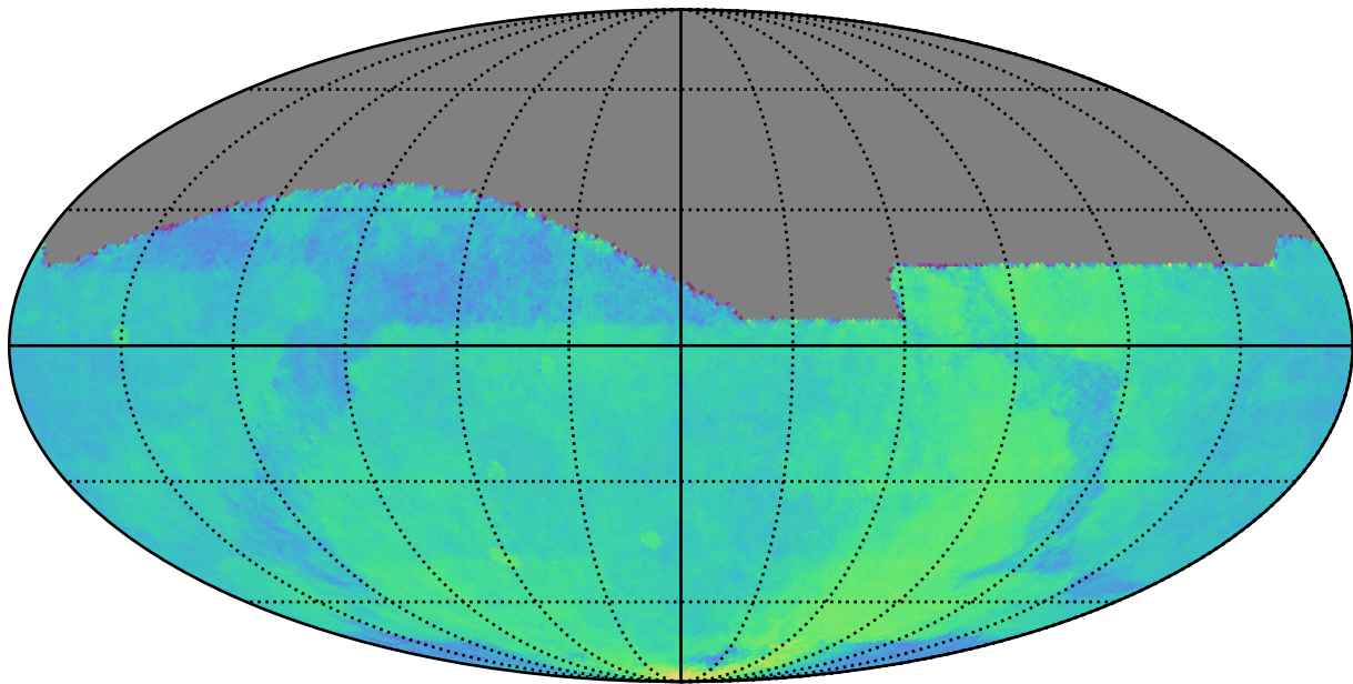
mw_roll_bulge_v3.3_10yrs All sky: Parallax Coverage @ 22.4
