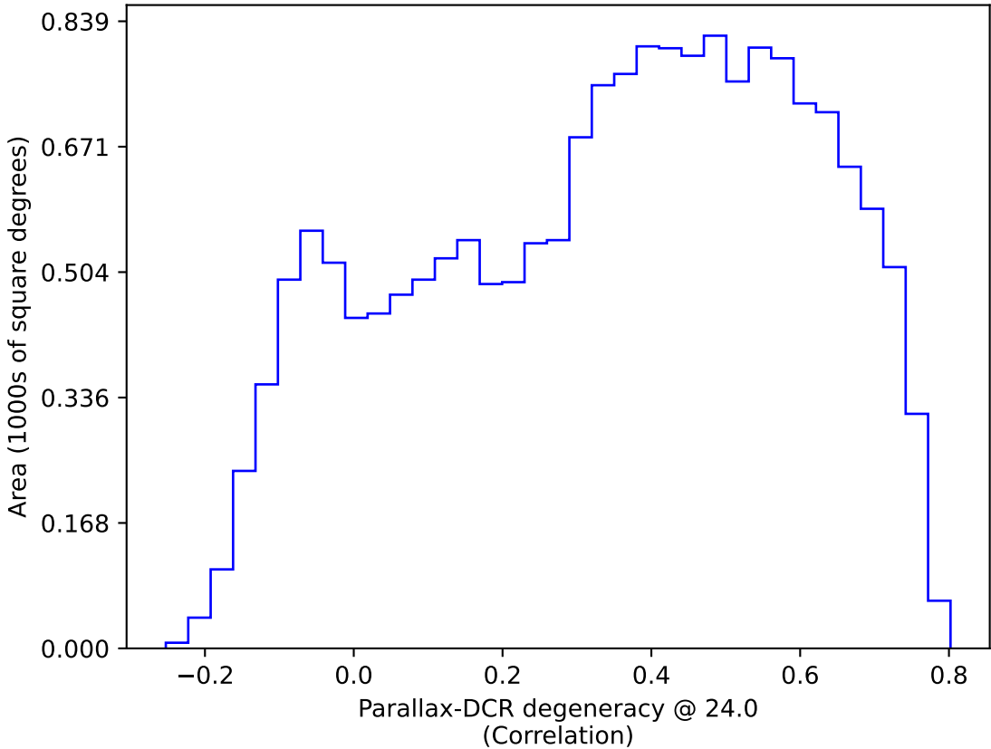
mw_roll_bulge_v3.3_10yrs WFD: Parallax-DCR degeneracy @ 24.0
