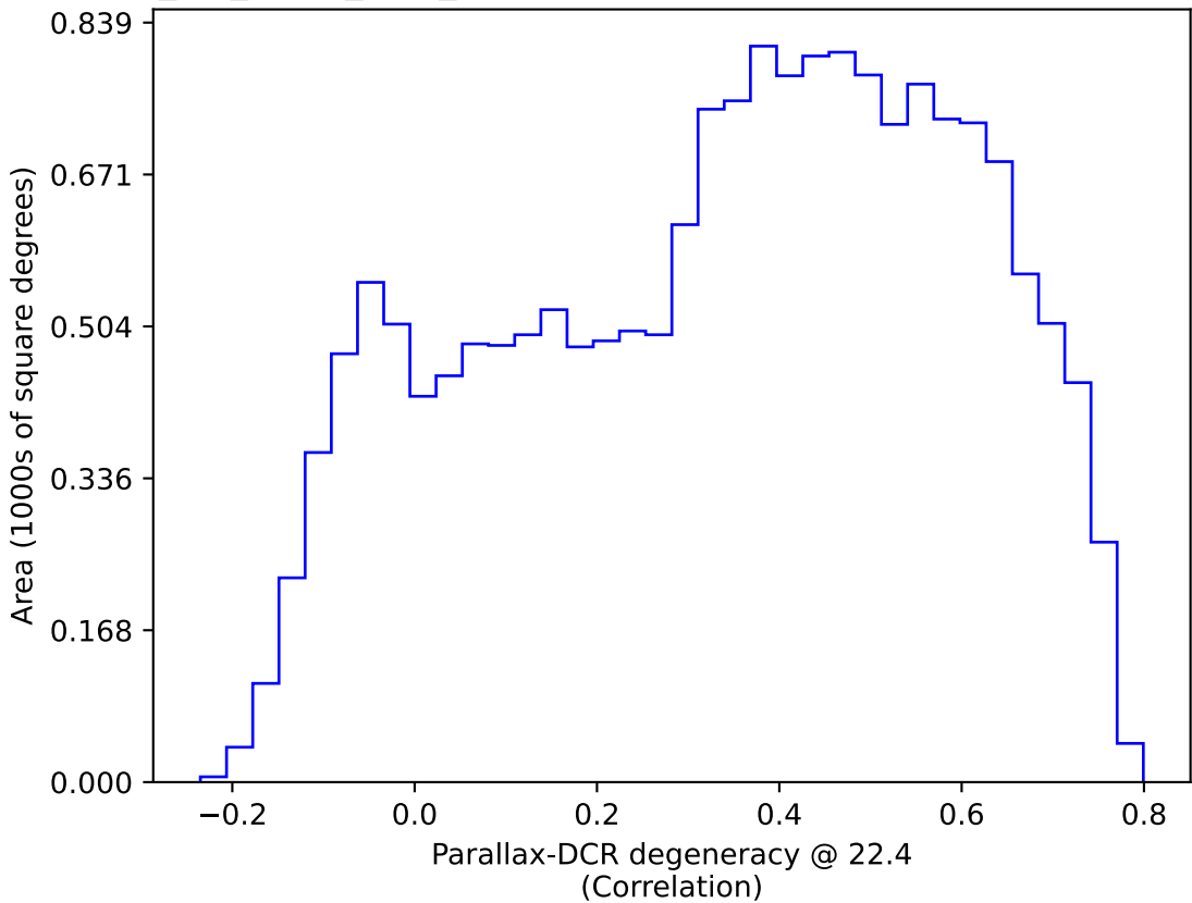
mw_roll_bulge_v3.3_10yrs WFD: Parallax-DCR degeneracy @ 22.4
