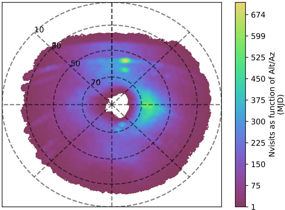
mw_roll_bulge_v3.3_10yrs u band: Nvisits as function of Alt/Az
