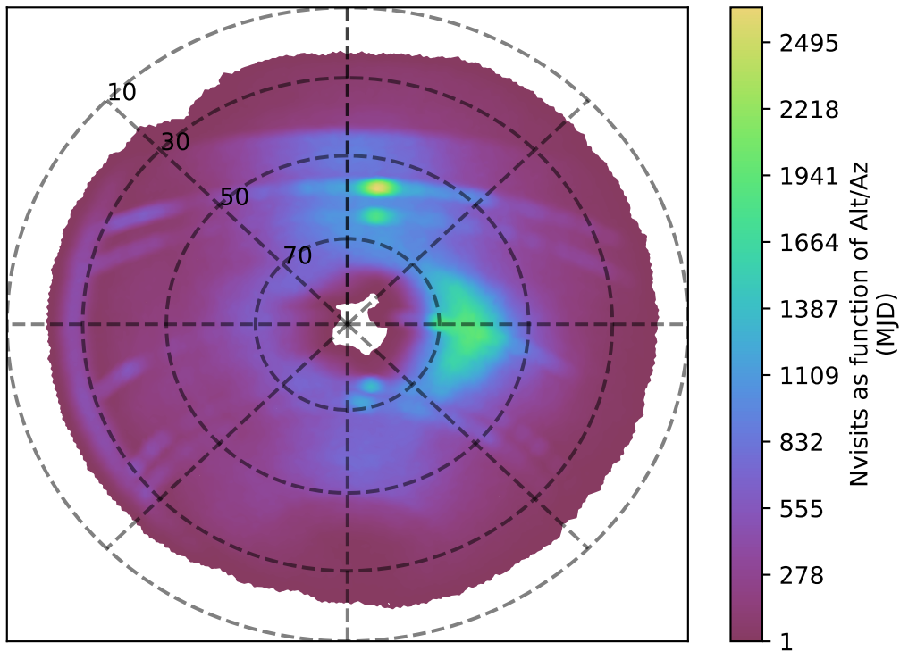
mw_roll_bulge_v3.3_10yrs r band: Nvisits as function of Alt/Az
