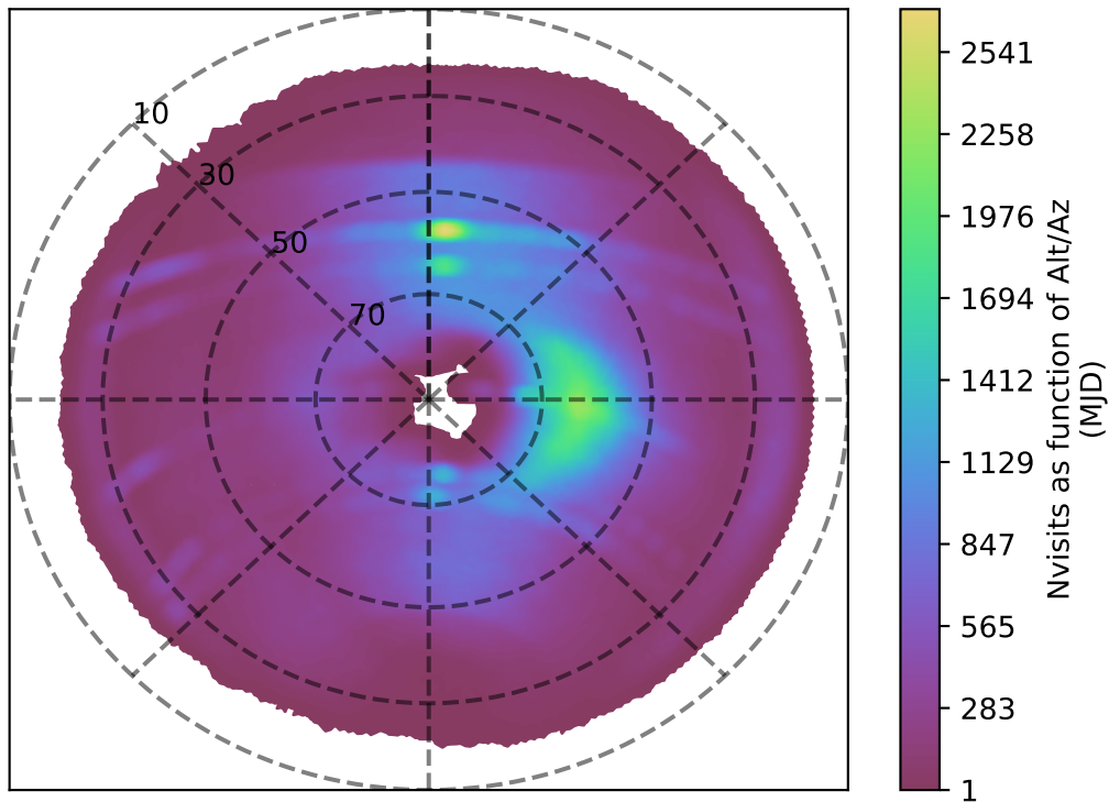
mw_roll_bulge_v3.3_10yrs i band: Nvisits as function of Alt/Az
