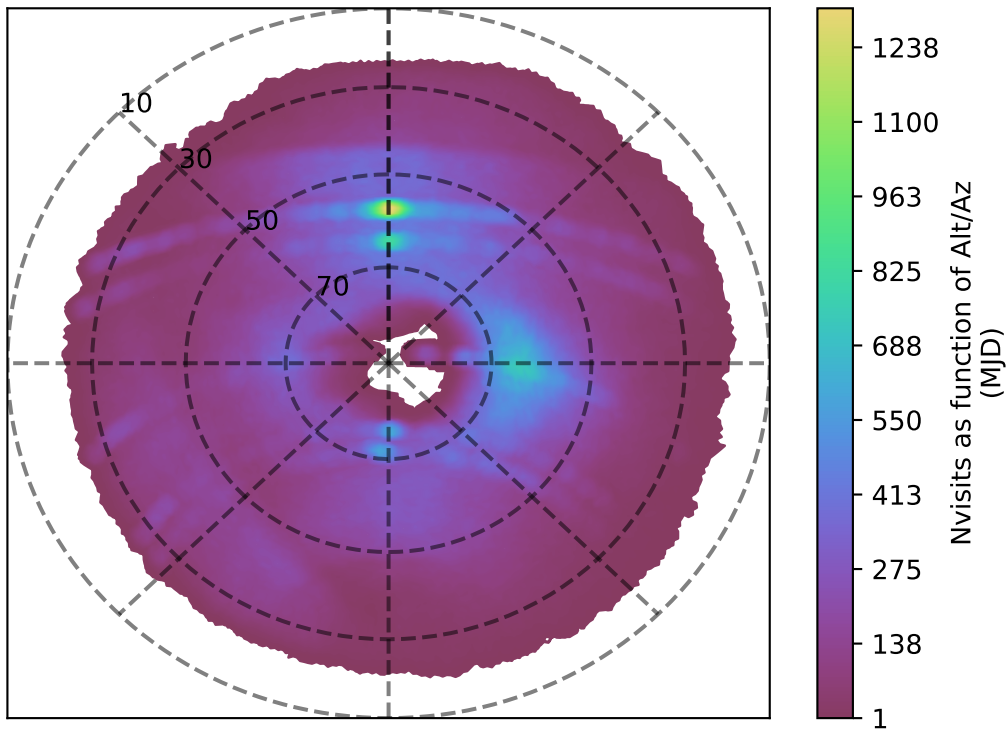
mw_roll_bulge_v3.3_10yrs g band: Nvisits as function of Alt/Az
