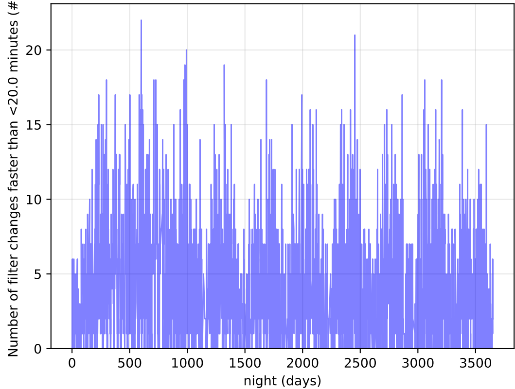
mw_roll_bulge_v3.3_10yrs Per Night: Number of filter changes faster than <20.0 minutes
