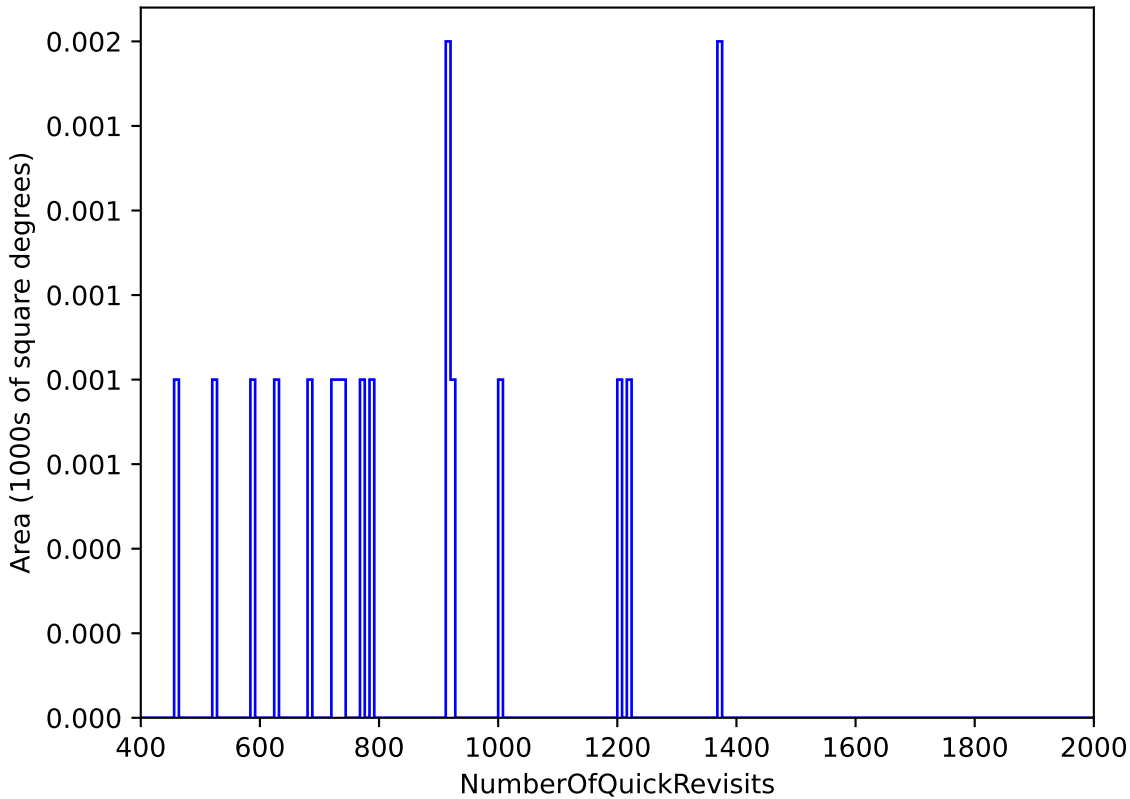
mw_roll_bulge_v3.3_10yrs WFD: NumberOfQuickRevisits
