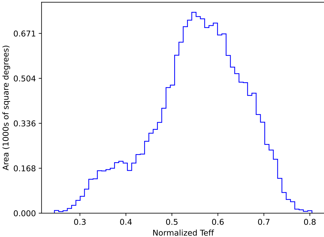
mw_roll_bulge_v3.3_10yrs WFD y band: Normalized Teff
