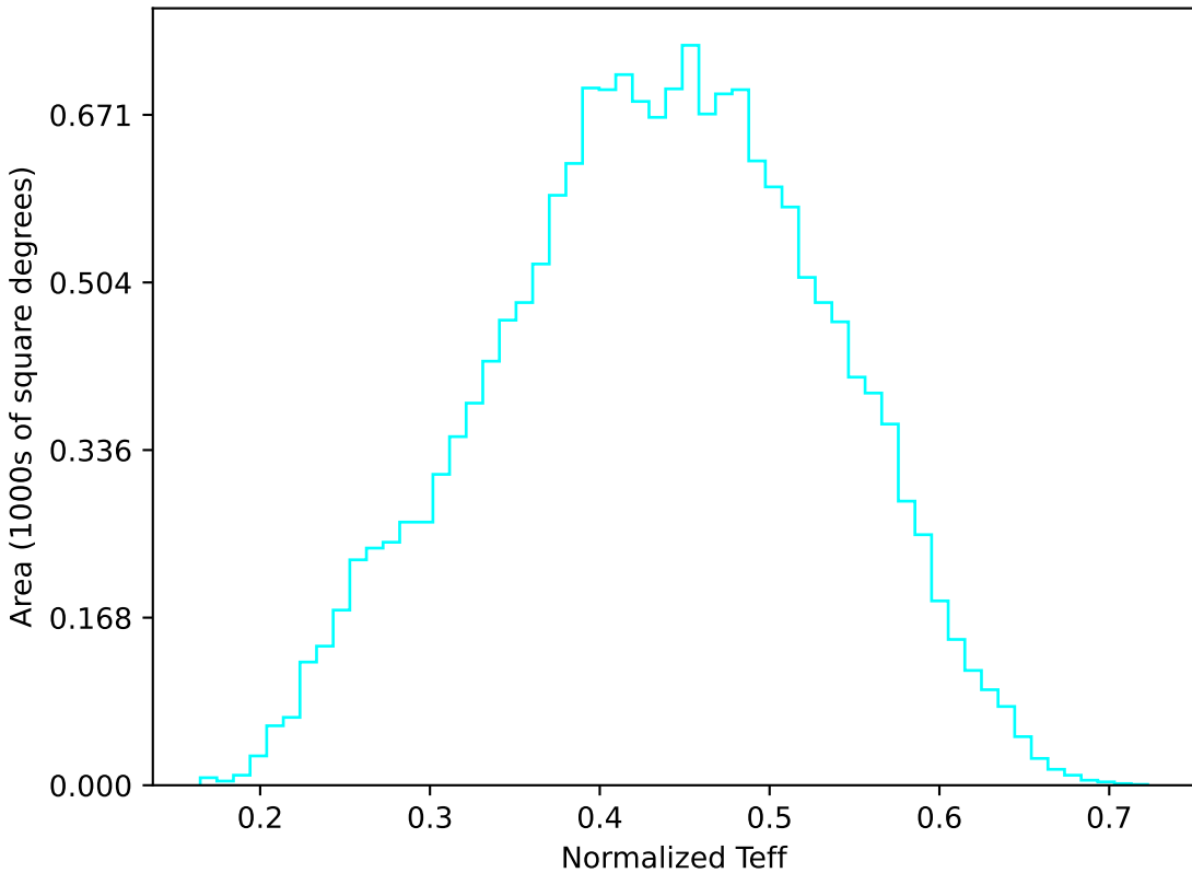
mw_roll_bulge_v3.3_10yrs WFD u band: Normalized Teff
