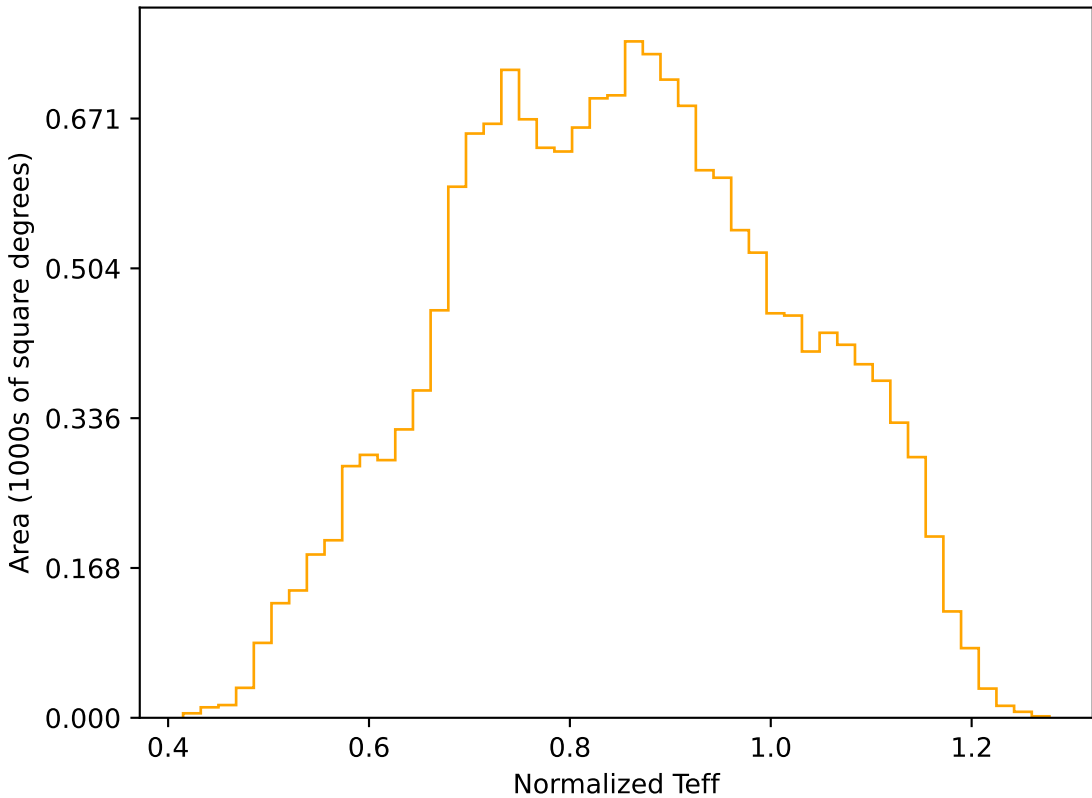
mw_roll_bulge_v3.3_10yrs WFD r band: Normalized Teff
