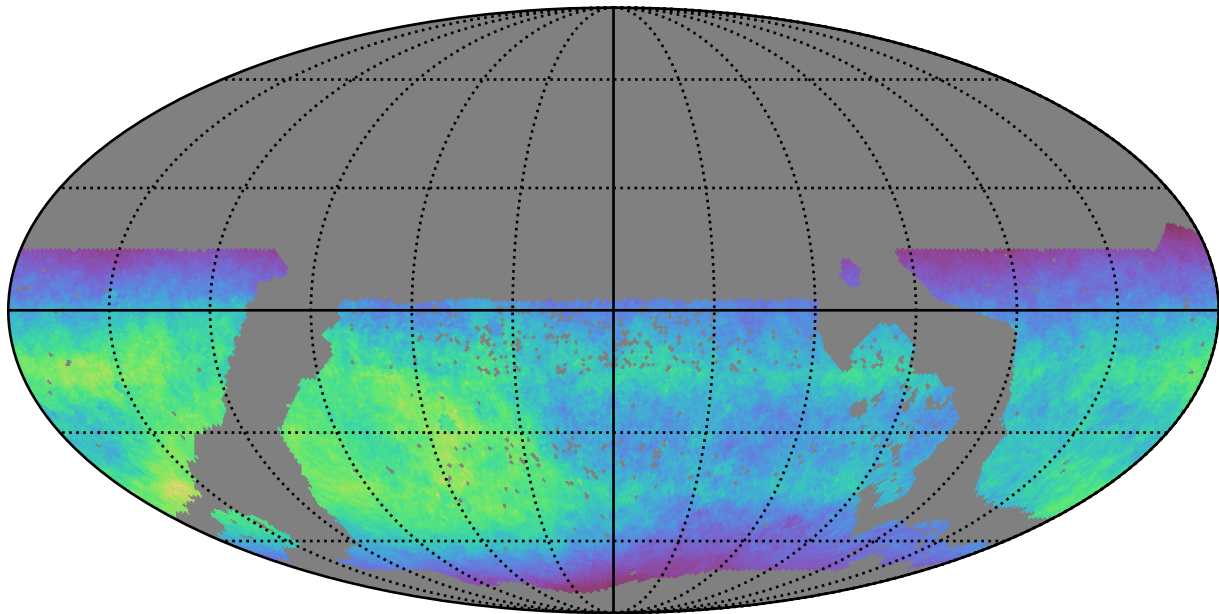
mw_roll_bulge_v3.3_10yrs WFD i band: Normalized Teff
