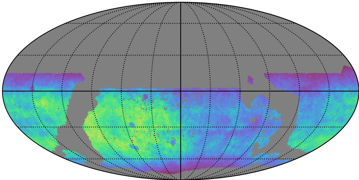
mw_roll_bulge_v3.3_10yrs WFD g band: Normalized Teff
