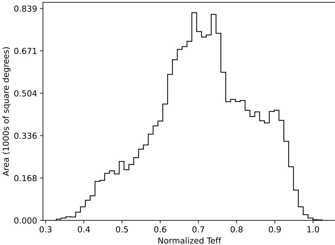
mw_roll_bulge_v3.3_10yrs WFD all bands: Normalized Teff
