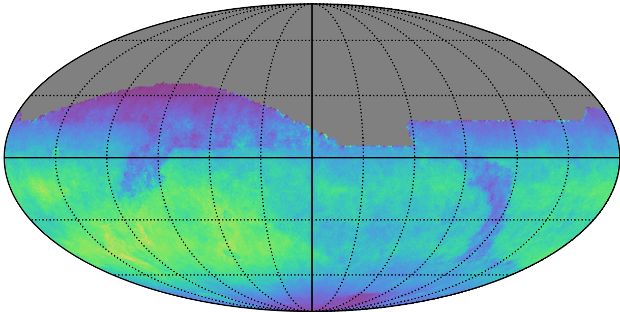
mw_roll_bulge_v3.3_10yrs All sky z band: Normalized Teff
