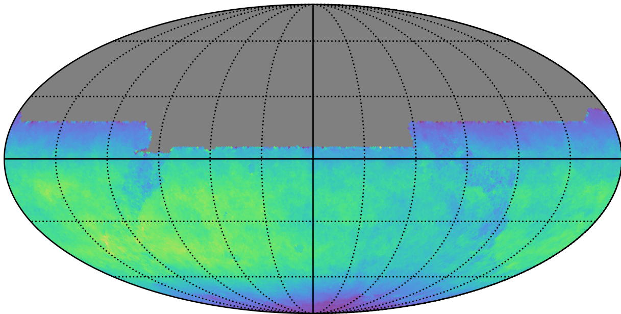
mw_roll_bulge_v3.3_10yrs All sky y band: Normalized Teff
