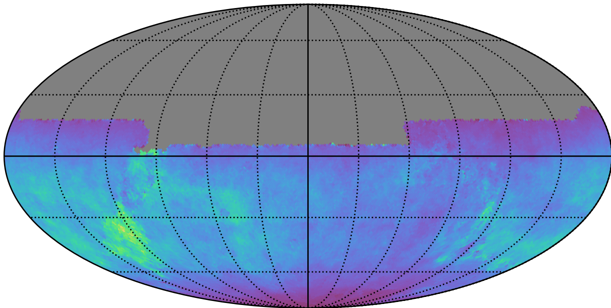
mw_roll_bulge_v3.3_10yrs All sky u band: Normalized Teff
