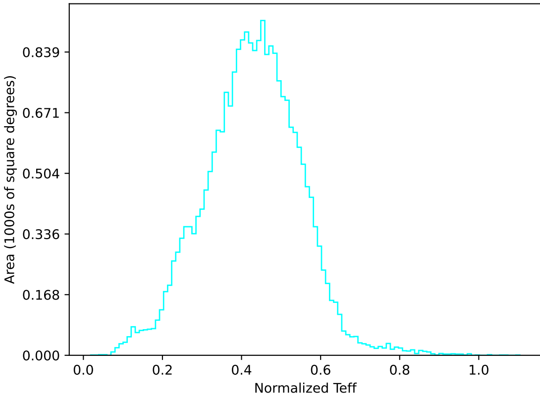
mw_roll_bulge_v3.3_10yrs All sky u band: Normalized Teff
