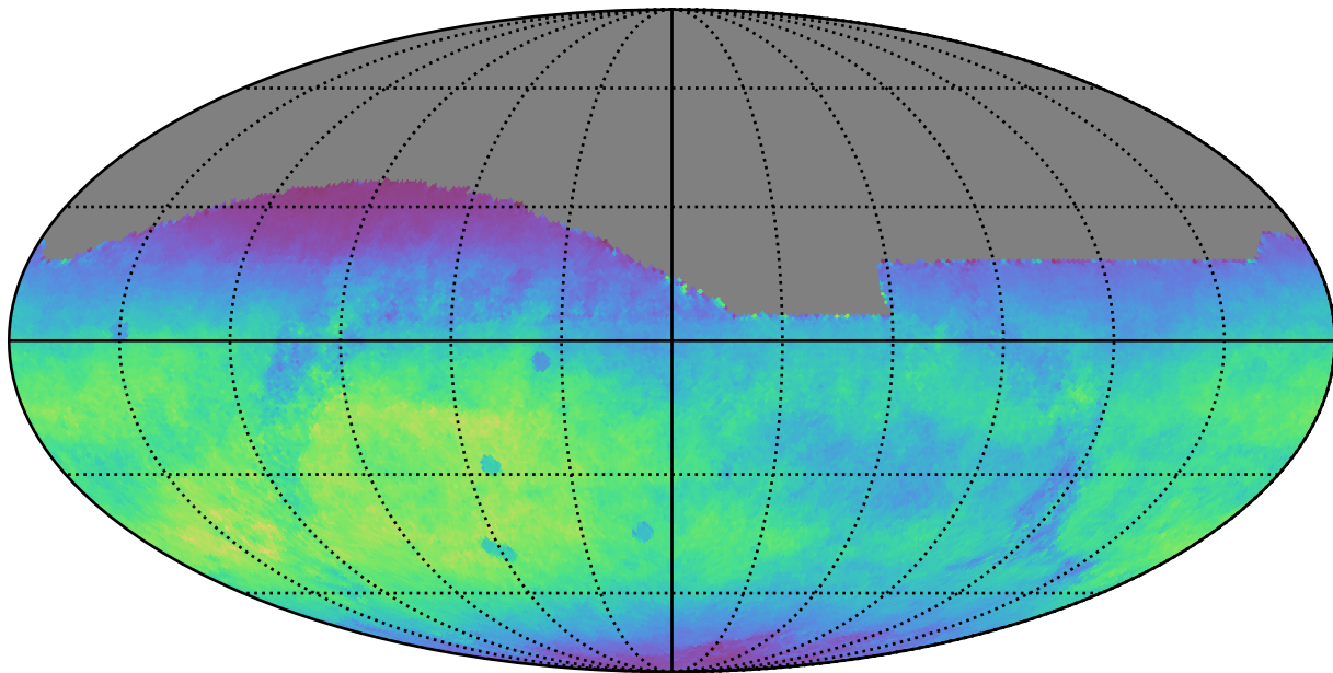
mw_roll_bulge_v3.3_10yrs All sky r band: Normalized Teff
