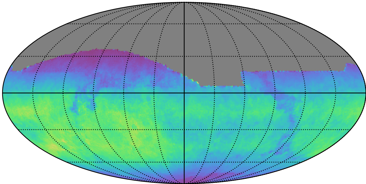
mw_roll_bulge_v3.3_10yrs All sky i band: Normalized Teff
