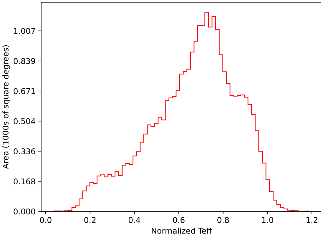
mw_roll_bulge_v3.3_10yrs All sky i band: Normalized Teff
