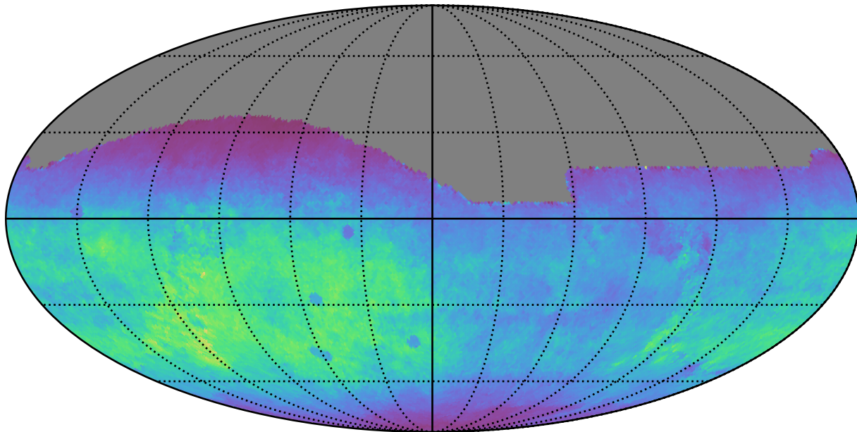
mw_roll_bulge_v3.3_10yrs All sky g band: Normalized Teff
