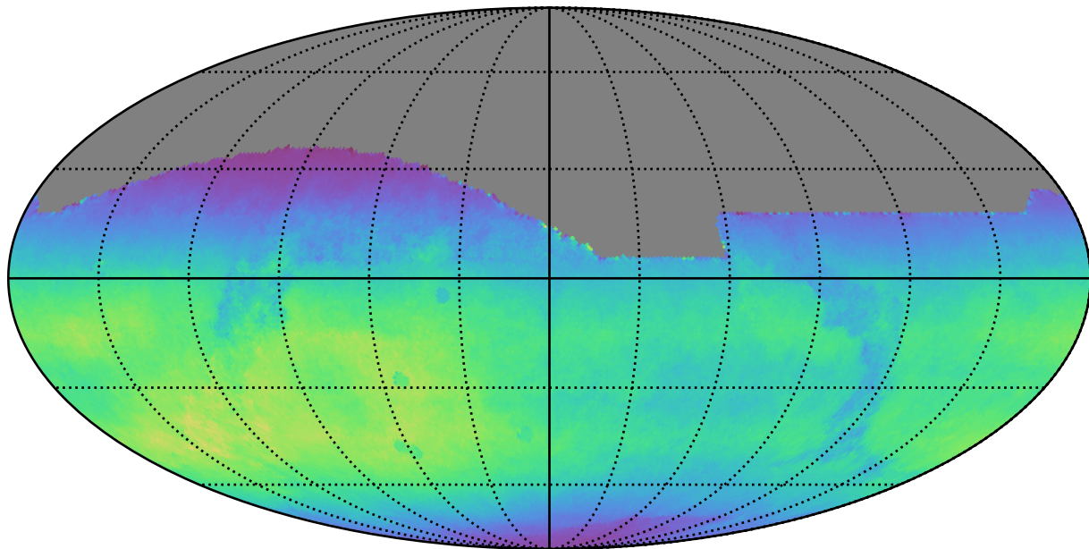
mw_roll_bulge_v3.3_10yrs All sky all bands: Normalized Teff
