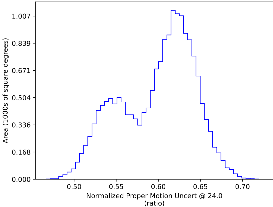
mw_roll_bulge_v3.3_10yrs WFD: Normalized Proper Motion Uncert @ 24.0
