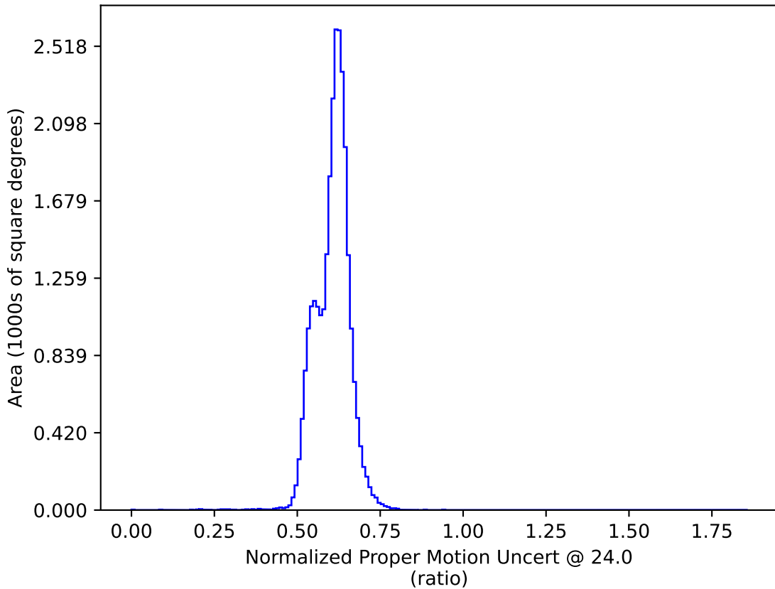
mw_roll_bulge_v3.3_10yrs All sky: Normalized Proper Motion Uncert @ 24.0
